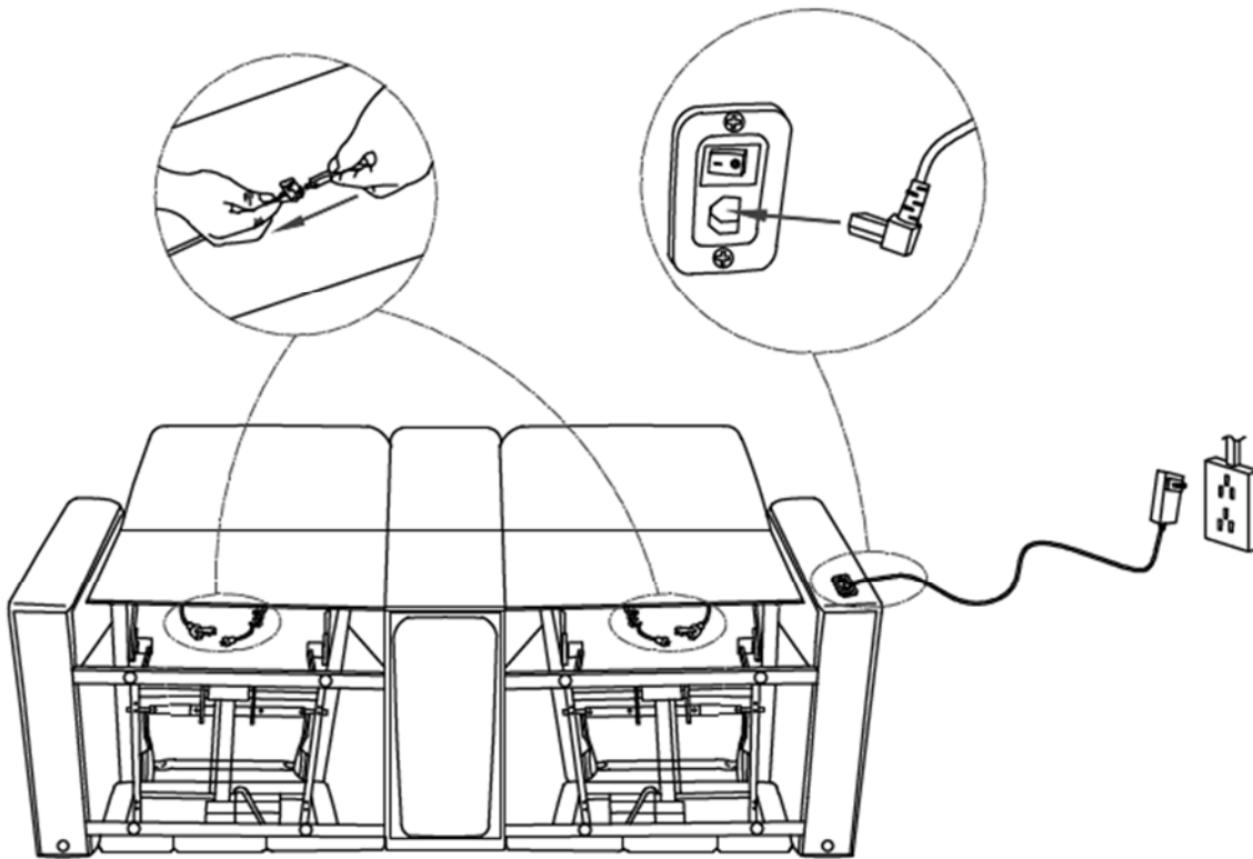
Power Transformer and Cord
